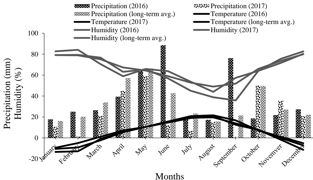
Figure 1. Some climate data of Yakutiye district of Erzurum Province in 2016, 2017, and long-term average (LTA).
